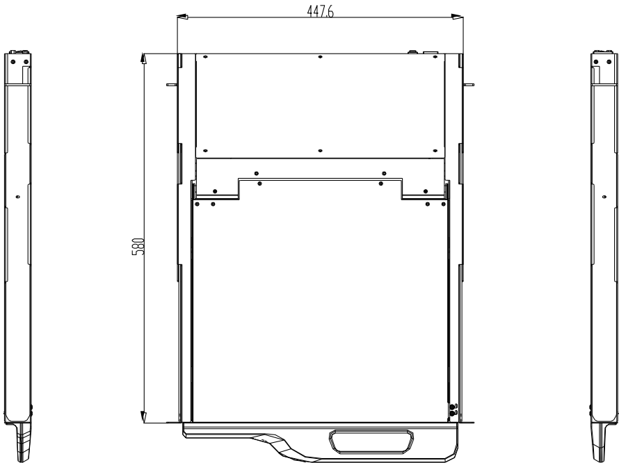
Rear of KVM-1732/1932ASL-M7/ULC
