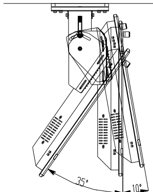
ROOF mount
